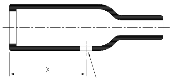
OPTION TO STANDARD PART FILLER PORT (CODE P1)
